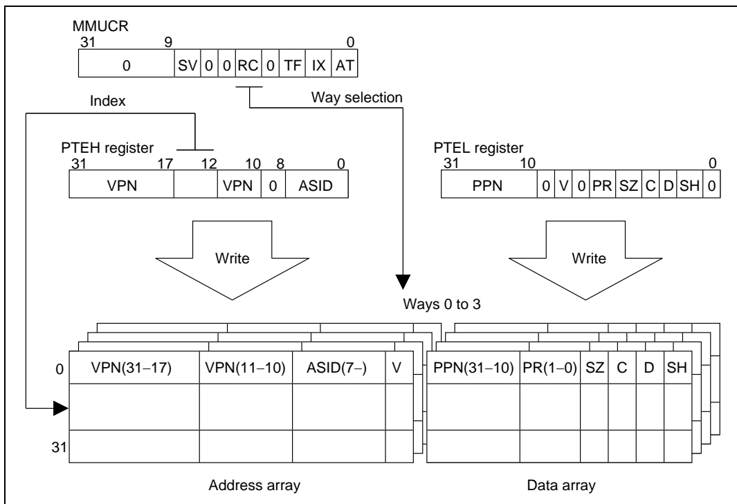
Figure 3.9 Operation of LDTLB Instruction
