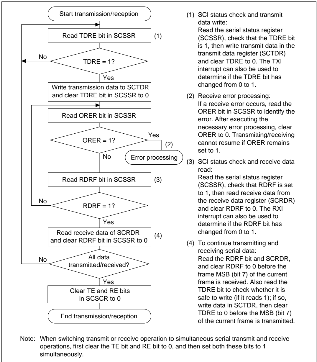
Figure 17.23 Sample Flowchart of Simultaneous Serial Transmit and Receive Operations
