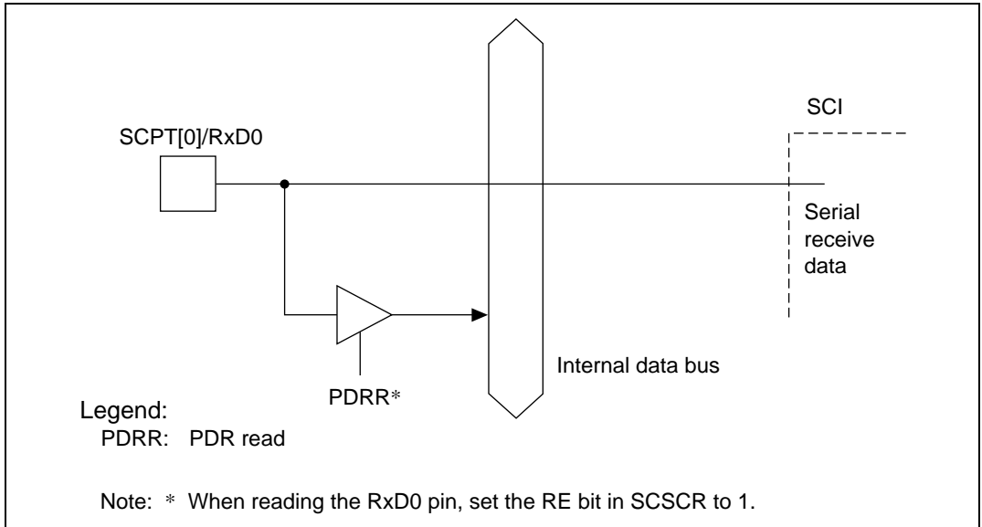
Figure 17.4 SCPT[0]/RxD0 Pin
