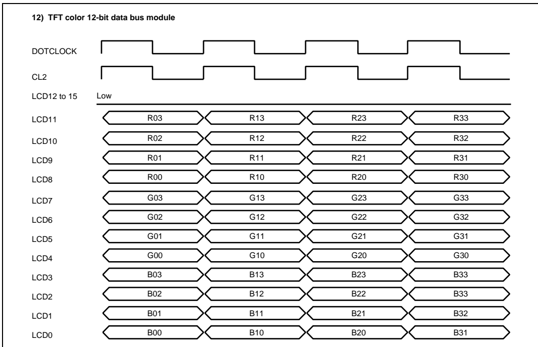
Figure 25.19 Clock and LCD Data Signal Example
