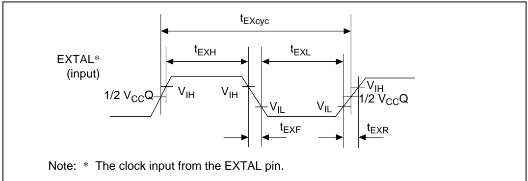
Figure 32.3 EXTAL Clock Input Timing
