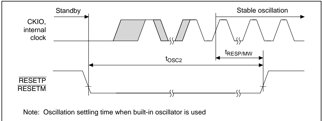
Figure 32.7 Oscillation Settling Time at Standby Return (Return by Reset)
