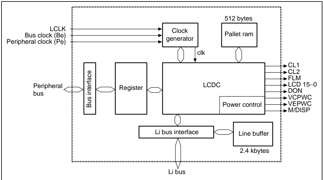
Figure 25.1 Block Diagram
