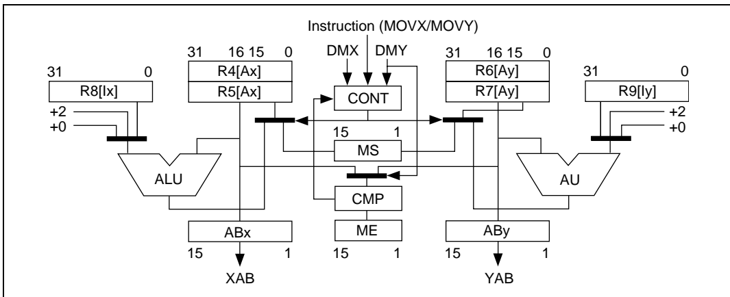
Figure 2.14 Modulo Addressing
