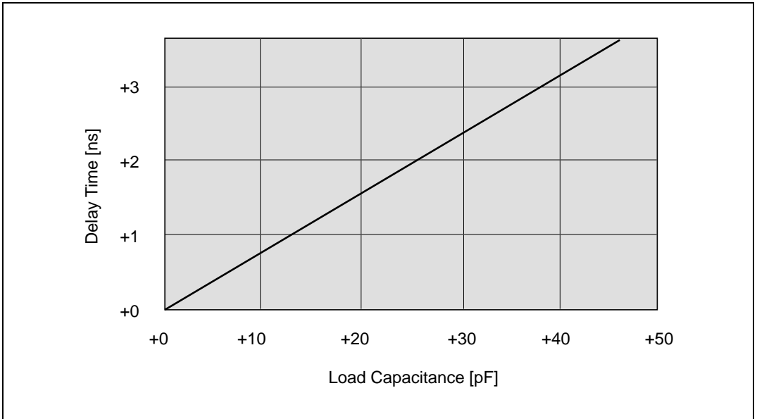
Figure 32.61 Load Capacitance vs. Delay Time
