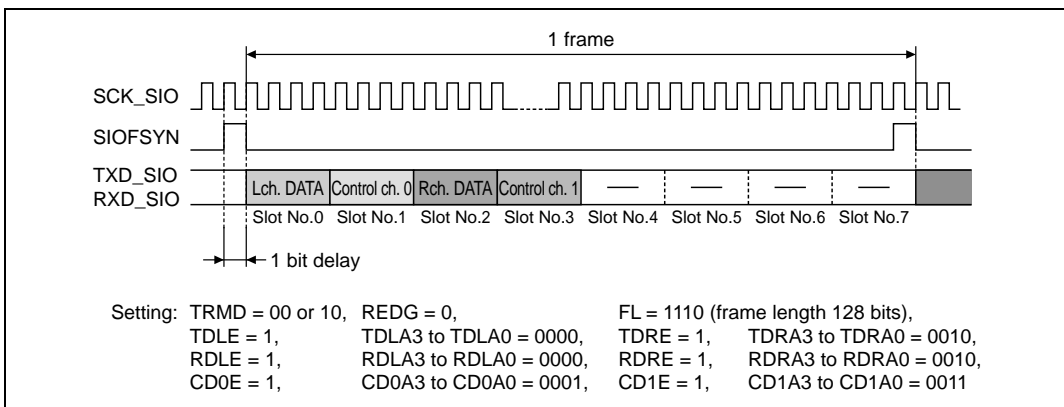
Figure 20.18 Transmit or Receive Timing (16 bits stereo—3)
