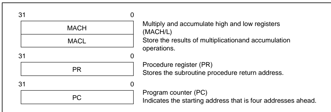
Figure 2.6 System Registers
