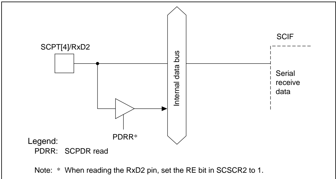
Figure 19.3 SCPT[4]/RxD2 Pin
