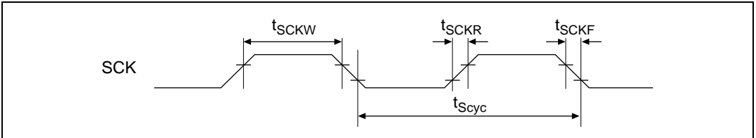
Figure 32.42 SCK Input Clock Timing
