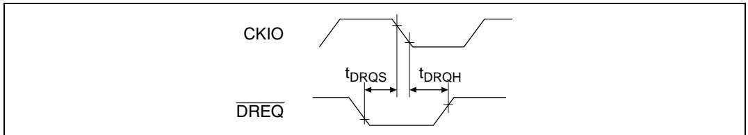
Figure 32.45 \overline{DREQ} Input Timing
