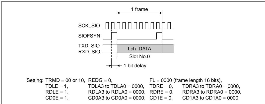
Figure 20.13 Transmit or Receive Timing (8 bits monaural—1)
