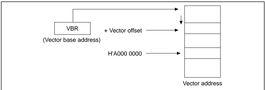
Figure 4.1 Vector Table
