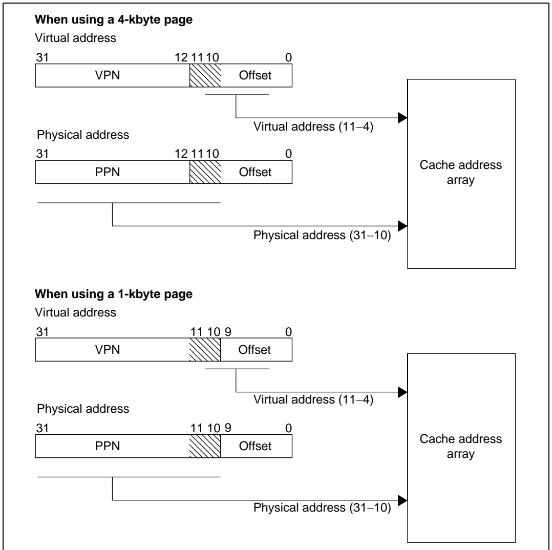
Figure 3.10 Synonym Problem
