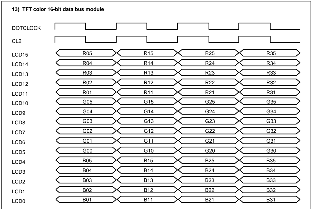
Figure 25.20 Clock and LCD Data Signal Example
