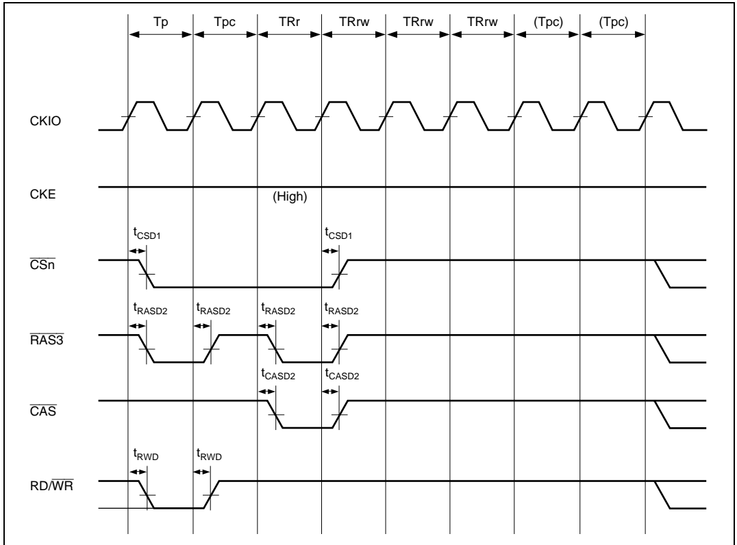
Figure 32.31 Synchronous DRAM Auto-Refresh Cycle ( TRAS = 1 , TPC = 1 )
