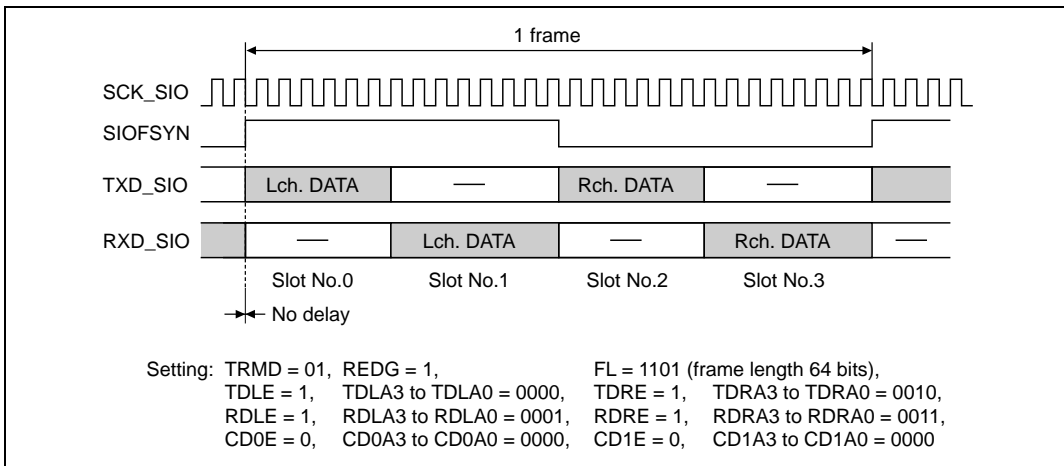
Figure 20.17 Transmit or Receive Timing (16 bits stereo—2)
