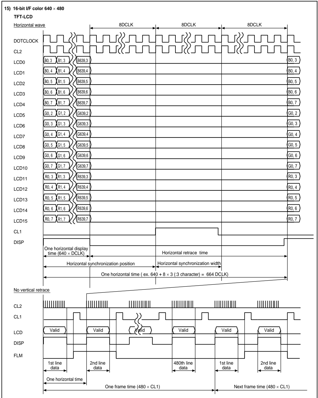
Figure 25.22 Clock and LCD Data Signal Example
