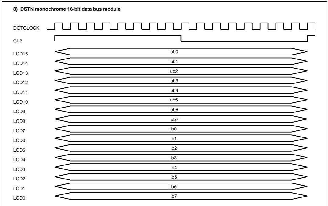
Figure 25.15 Clock and LCD Data Signal Example
