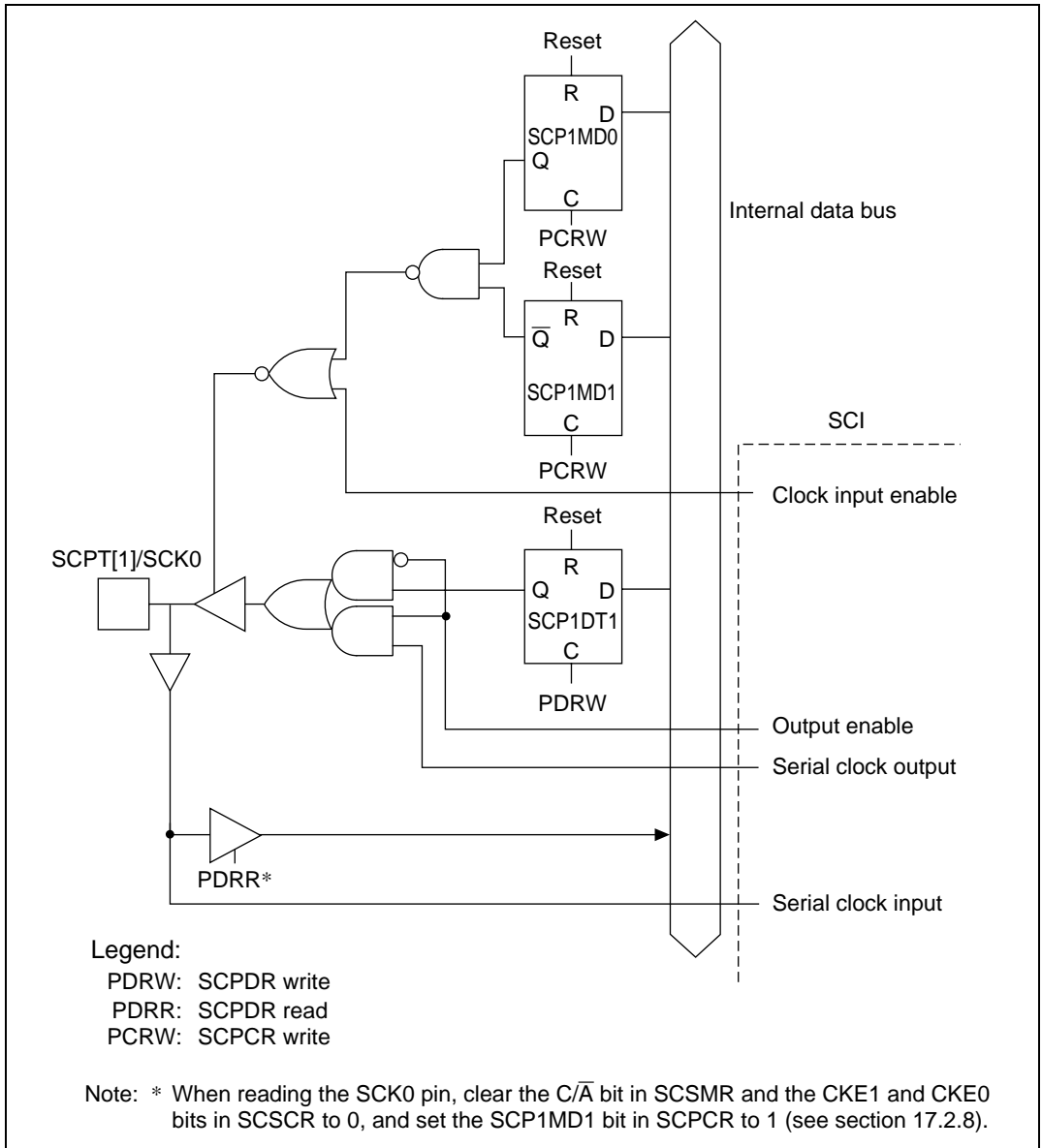
Figure 17.2 SCPT[1]/SCK0 Pin
