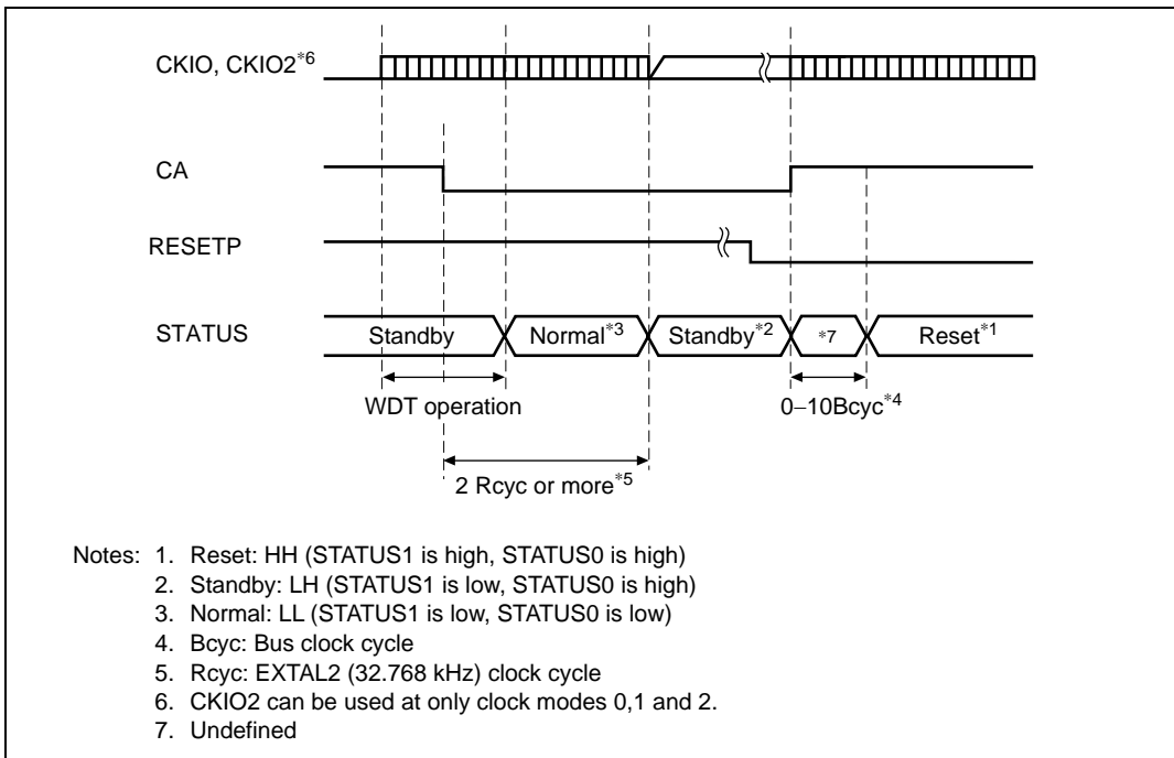
Figure 9.11 Hardware Standby Mode Timing (CA = Low during WDT Operation while Standby Mode is Cleared)
