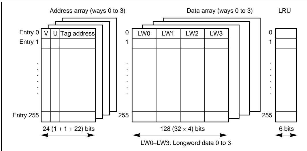
Figure 5.1 Cache Structure
