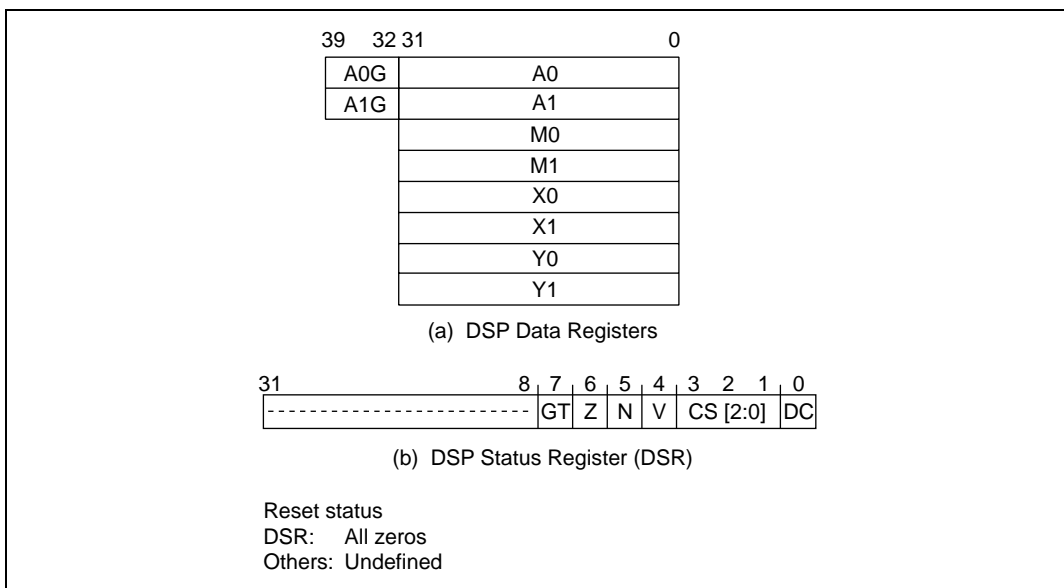
Figure 2.7 DSP Registers
