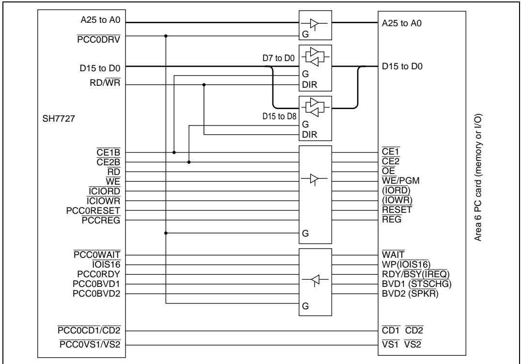
Figure 30.4 SH7727 Interface
