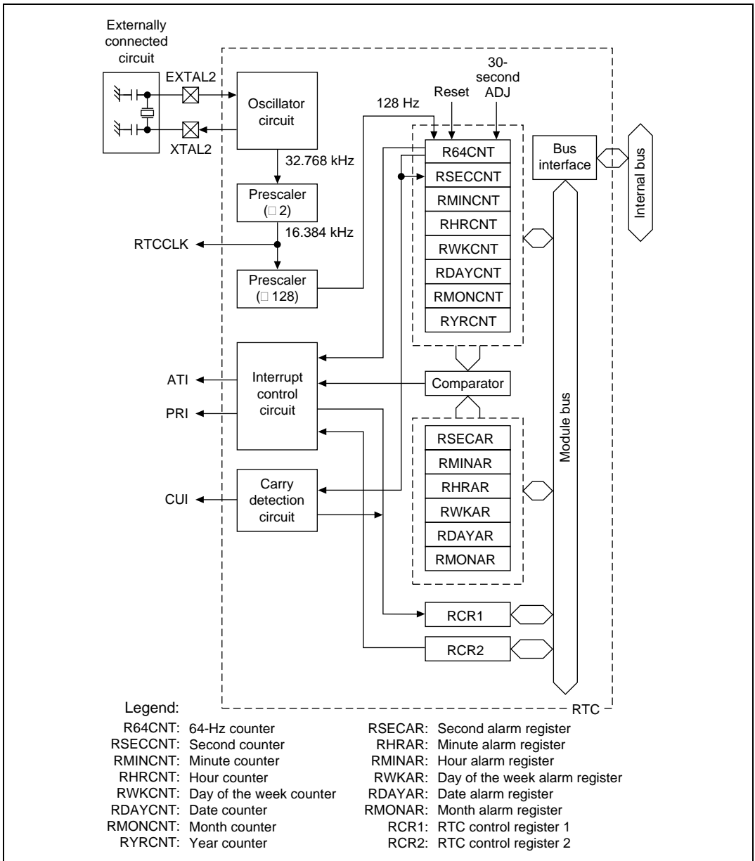
Figure 16.1 RTC Block Diagram
