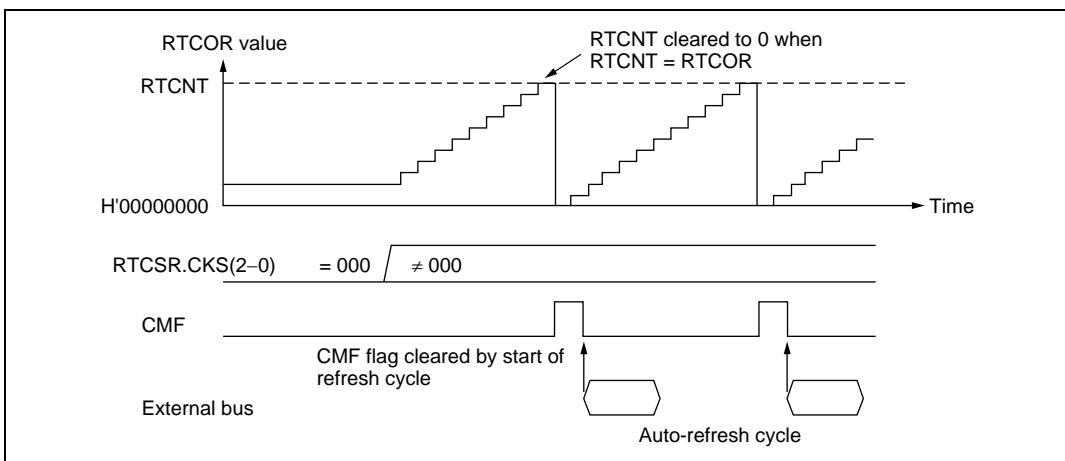
Figure 12.18 Auto-Refresh Operation
