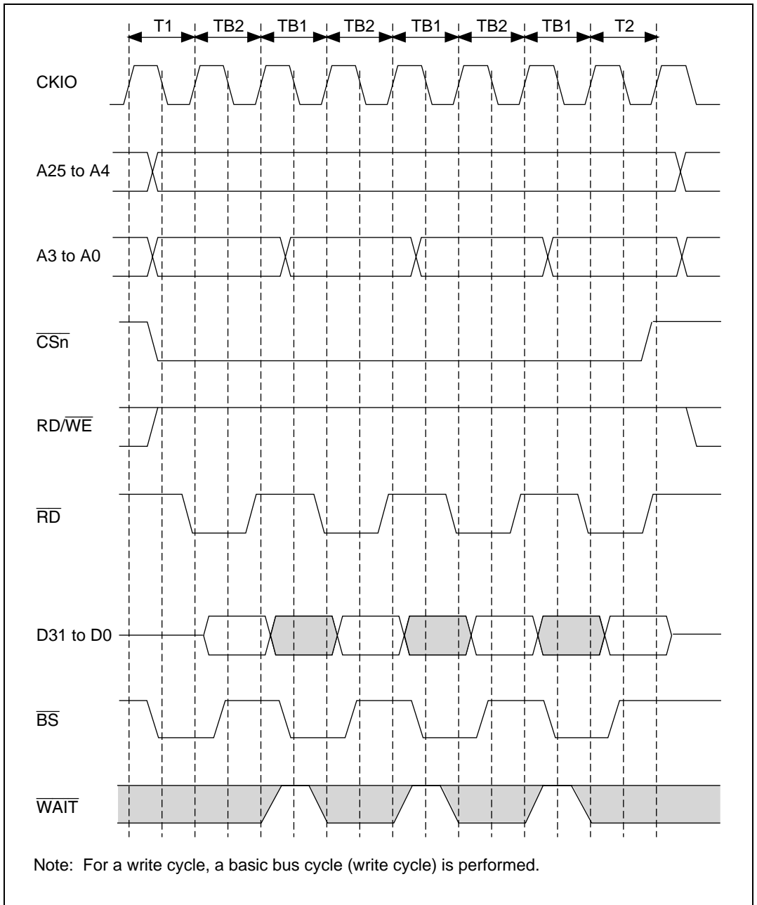
Figure 12.23 Burst ROM Basic Access Timing
