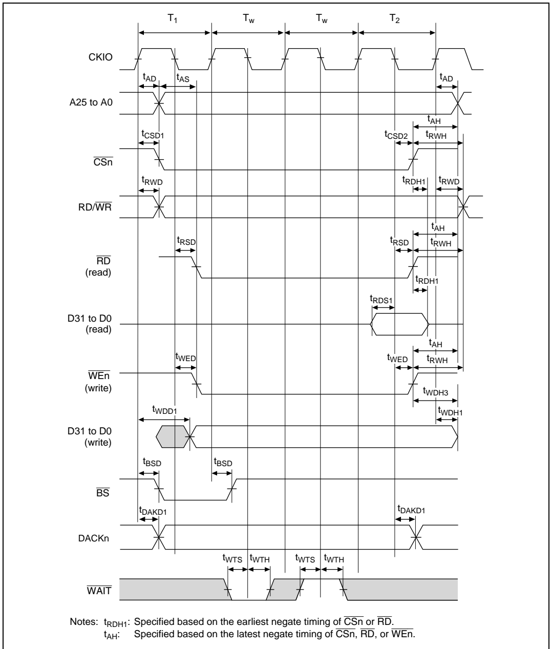
Figure 32.19 Basic Bus Cycle (External Wait, WAITSEL = 1)
