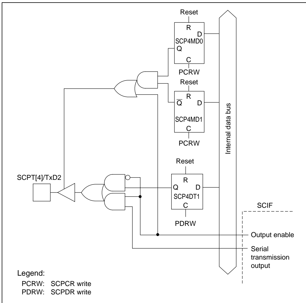
Figure 19.2 SCPT[4]/TxD2 Pin
