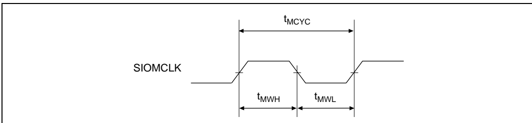
Figure 32.52 SIOMCLK Input Timing
