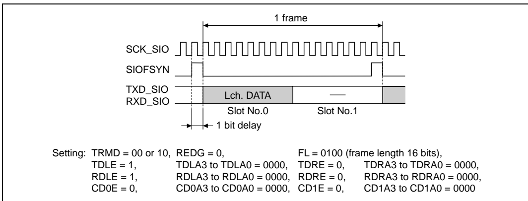
Figure 20.14 Transmit or Receive Timing (8 bits monaural—2)
